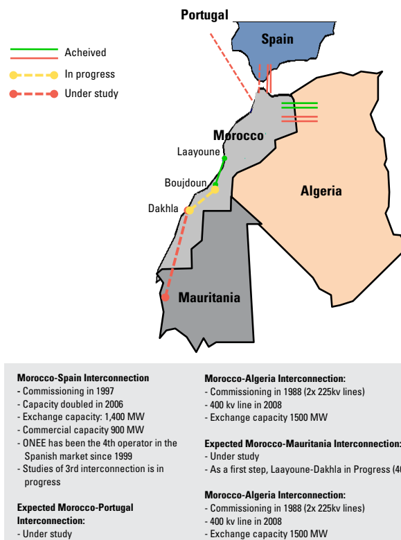
Figure 6: Moroccan electrical interconnections
