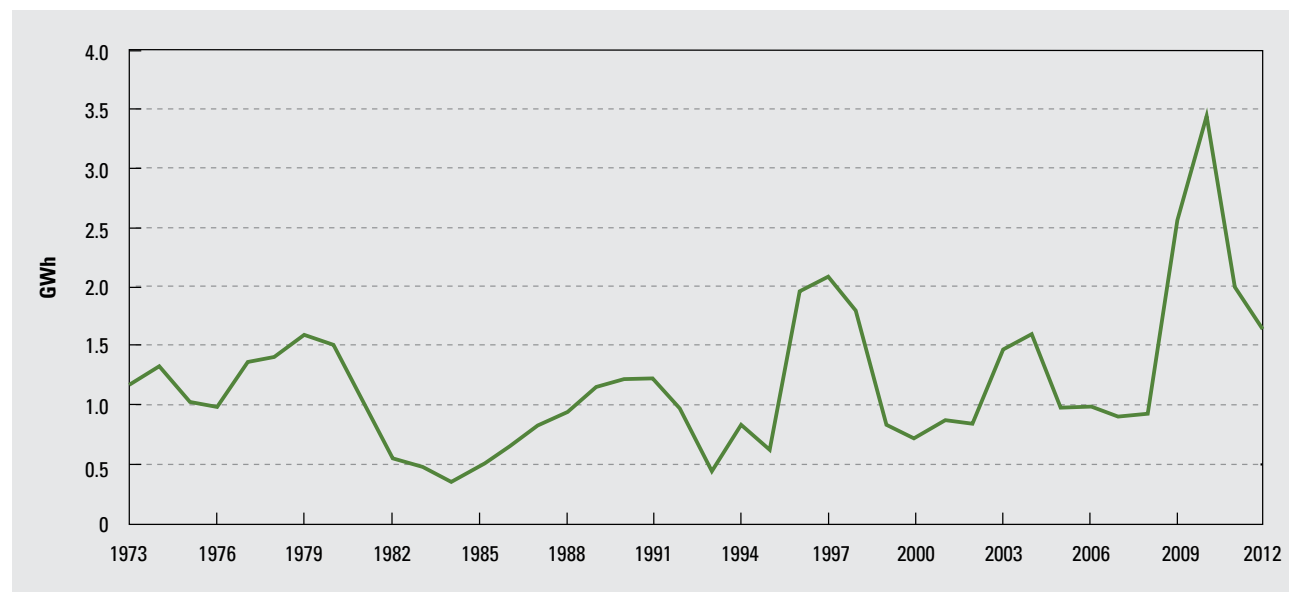
Figure 18: Variability of hydropower generation in Morocco, 1973–2012
