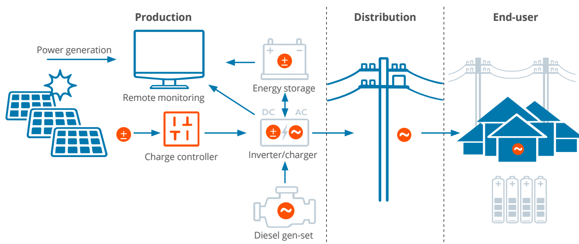
Figure 2 Components of a solar mini-grid system
